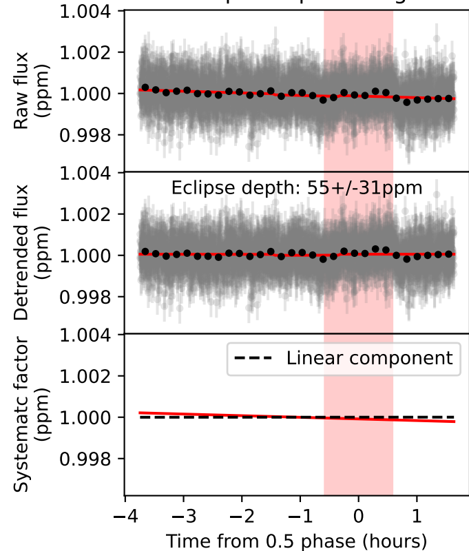
Eclipse depth fitting
